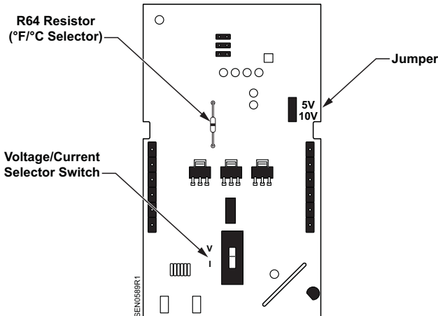
Figure 4. Circuit Board (Located inside Room Unit Cover.)
