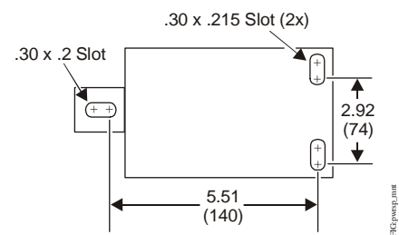
Power Supply Mounting Dimensions, in. (mm)
