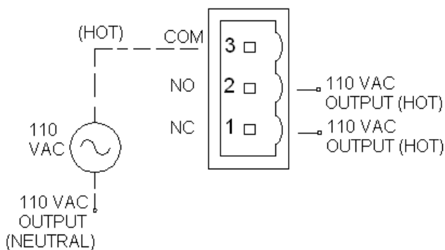
Figure 5 – Diagram of Electrical Connections
