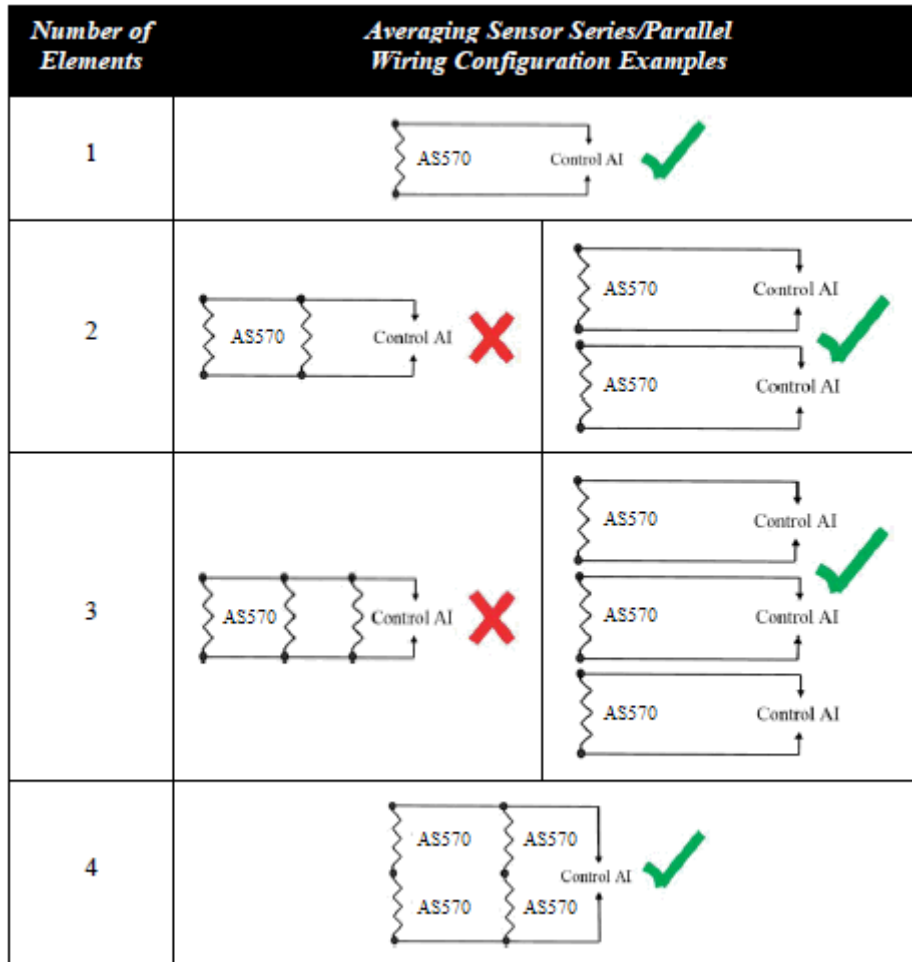
Figure 7 – Series-Parallel Wiring Configuration Examples
