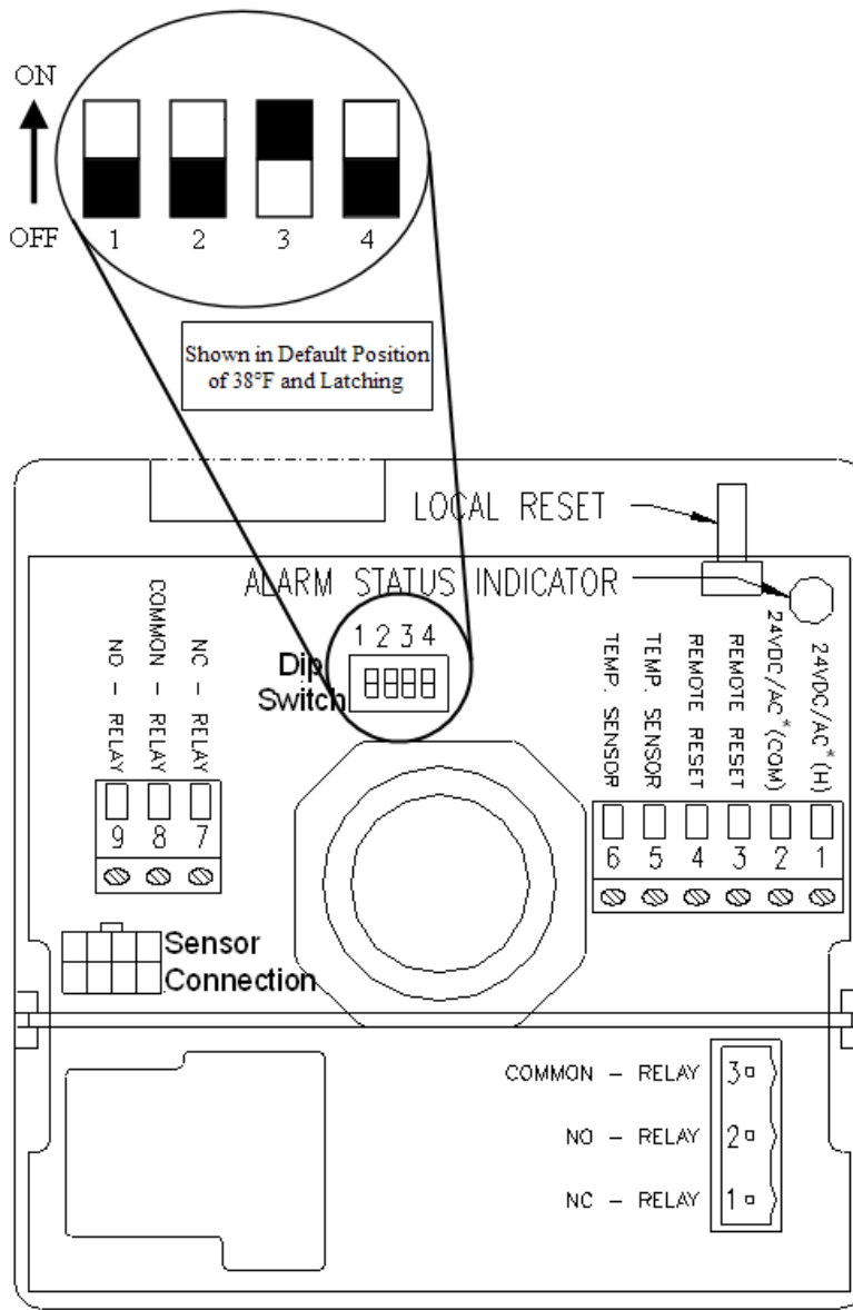
Figure 2 – Setpoint Adjustment Diagram
