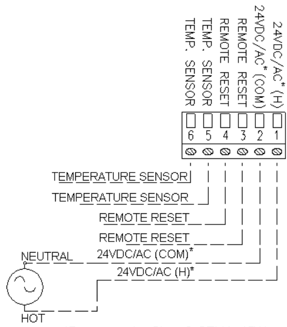
Figure 5 – Diagram of Electrical Connections
