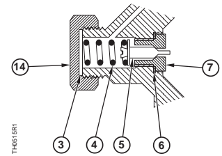
Figure 5. Exhaust Valve.
