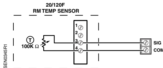
Figure 4. Wiring Example.
