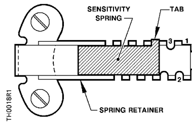
Figure 10. Sensitivity Spring Setting.
