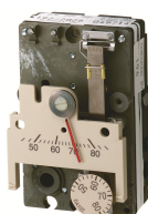
192S Single Setpoint Pneumatic Room Thermostat
