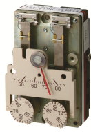
193HC Hesitation Free Energy Band Pneumatic Room Thermostat
