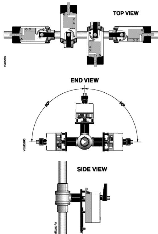
Figure 4. Mounting Positions.
