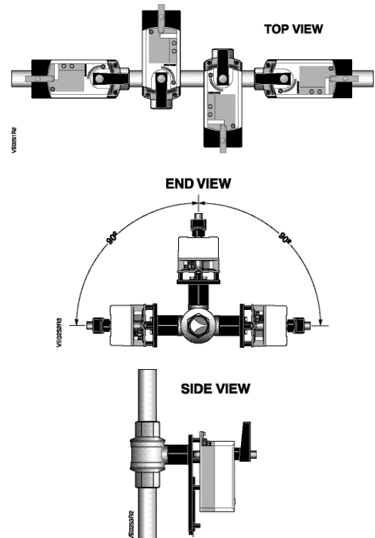
Figure 4. Mounting Positions.
