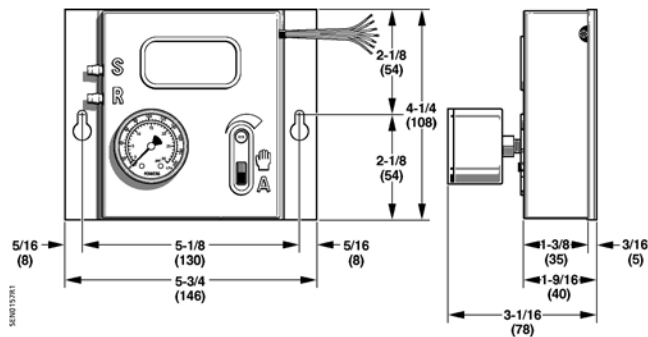
545 AO-P Transducer
