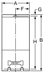
Figure 2 Class 8536
