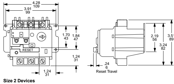
Size 2 Devices
