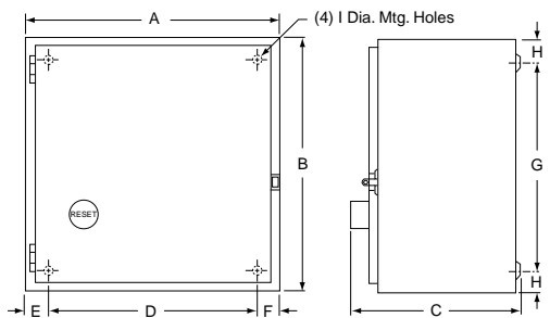
Figure 16.11: NEMA 1
