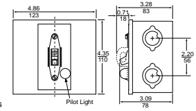
Jumbo (Class 9991 Type KE2, see )
