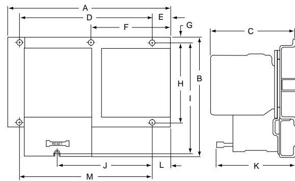
Figure 16.10: Class 8736 Starter, Open Type
