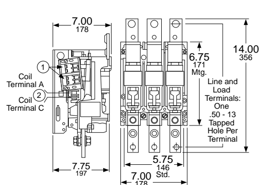
Dimensions for Class 8502 Type VH Size 6
