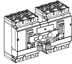
Interlocking with Toggle Control
