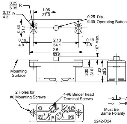
9007AO, Single-Pole Snap Switch
