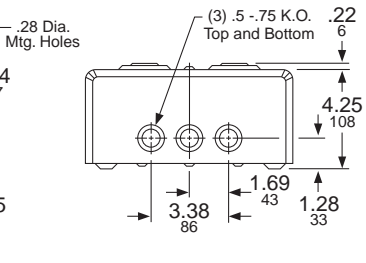
Classes 2511, 2512, Types M & T Sizes M-0 and M-1 NEMA 1 General Purpose Enclosure Approximate Shipping Weight: 9 lb
