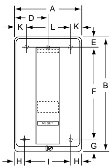
Figure 1 Dimensions: in. mm
