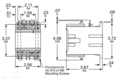
Type DPA—2 and 3-Pole 50 and 60 Full Load Amperes
