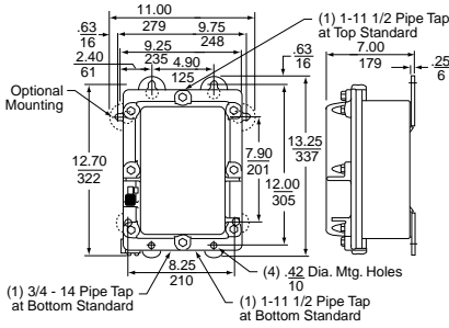
Bolted Cover, Cast Iron Enclosure, NEMA Size 0 and 1 (weight: 59 lb)
