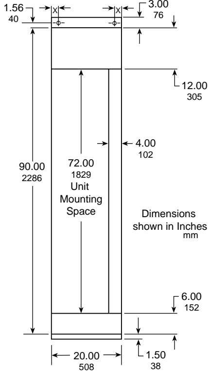
20-in. (508 mm)-wide Section with Standard Vertical Wireway
