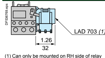
LRD01-35 and LRD313-365 Remote tripping or electrical reset
