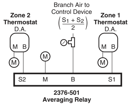
Figure 1 Typical Application.
