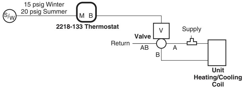
Figure 7 2218-133 Typical Application.
