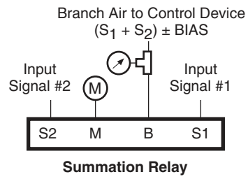
Figure 3 Typical Application.
