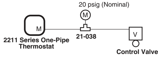
Figure 1 2211 Typical Application.
