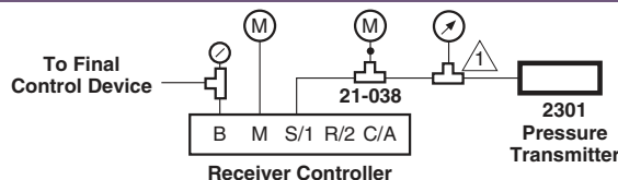
Figure 1 Typical Piping Diagram.
