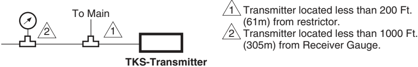
Figure 1 Typical Application.
