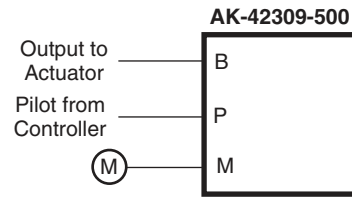
Figure 1 Piping Connections.
